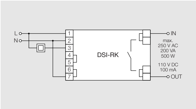
DSI-RK switch DIM
