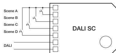
single momentary switch
